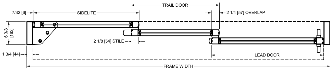
HORIZONTAL SECTION
