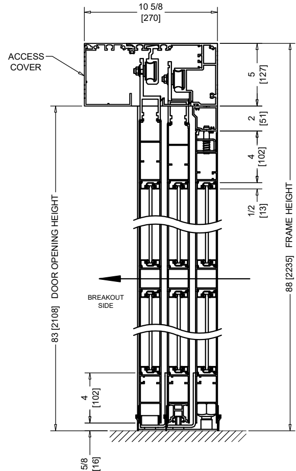
VERTICAL SECTION
