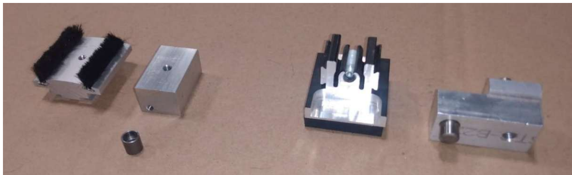
Old Stop Pin Assembly
