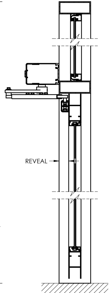
VERTICAL SECTION CENTER PIVOT OPTION OR BUTT/OFFSET PIVOT W/ REVEAL
