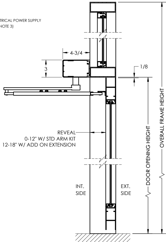
VERTICAL SECTION BUTT/OFFSET PIVOT OPTION
