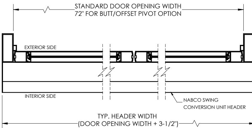
HORIZONTAL SECTION
