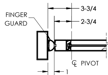
HINGE JAMB AT CENTER PIVOT OPTION
