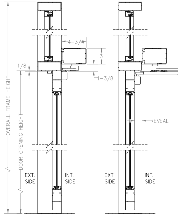
VERTICAL SECTION BUTT/OFFSET PIVOT OPTION
