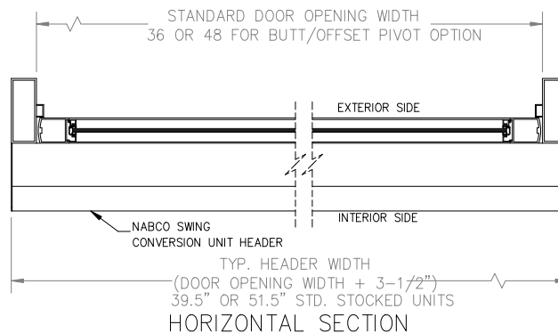
HORIZONTAL SECTION
