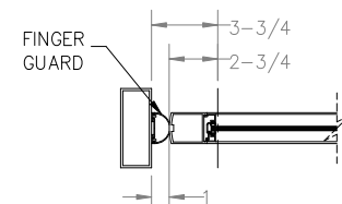
HINGE JAMB AT CENTER PIVOT OPTION
