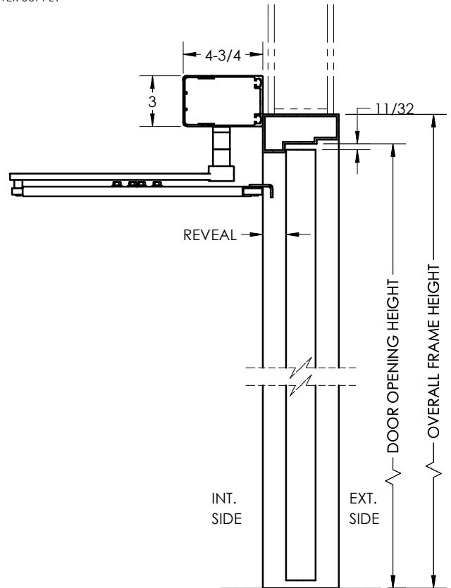
VERTICAL SECTION BUTT/OFFSET
