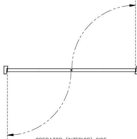
OPERATOR (INTERIOR) SIDE INTERIOR ELEVATION/PLAN
