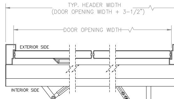
HORIZONTAL SECTION
