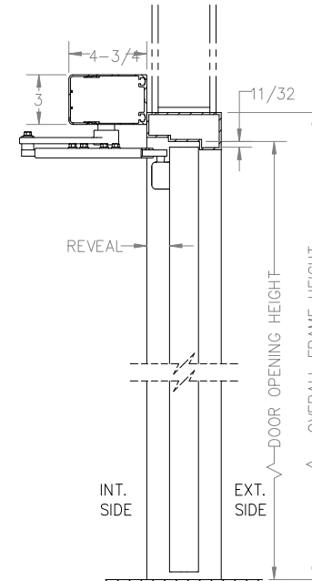
VERTICAL SECTION BUTT/OFFSET
