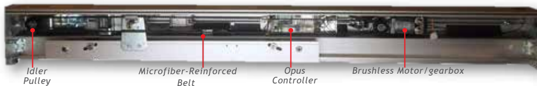
GT1175 Header Diagram with Opus Controller
