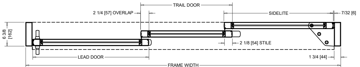
HORIZONTAL SECTION
