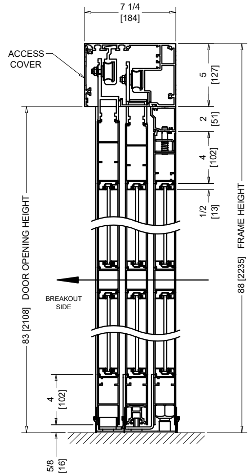
VERTICAL SECTION
