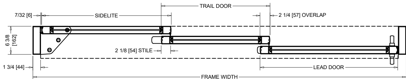
HORIZONTAL SECTION
