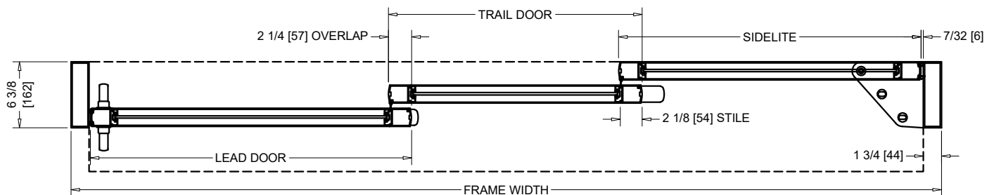
HORIZONTAL SECTION
