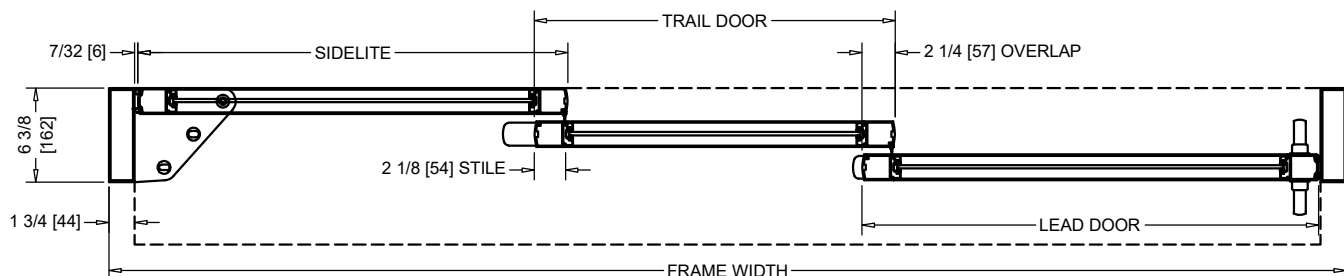
HORIZONTAL SECTION
