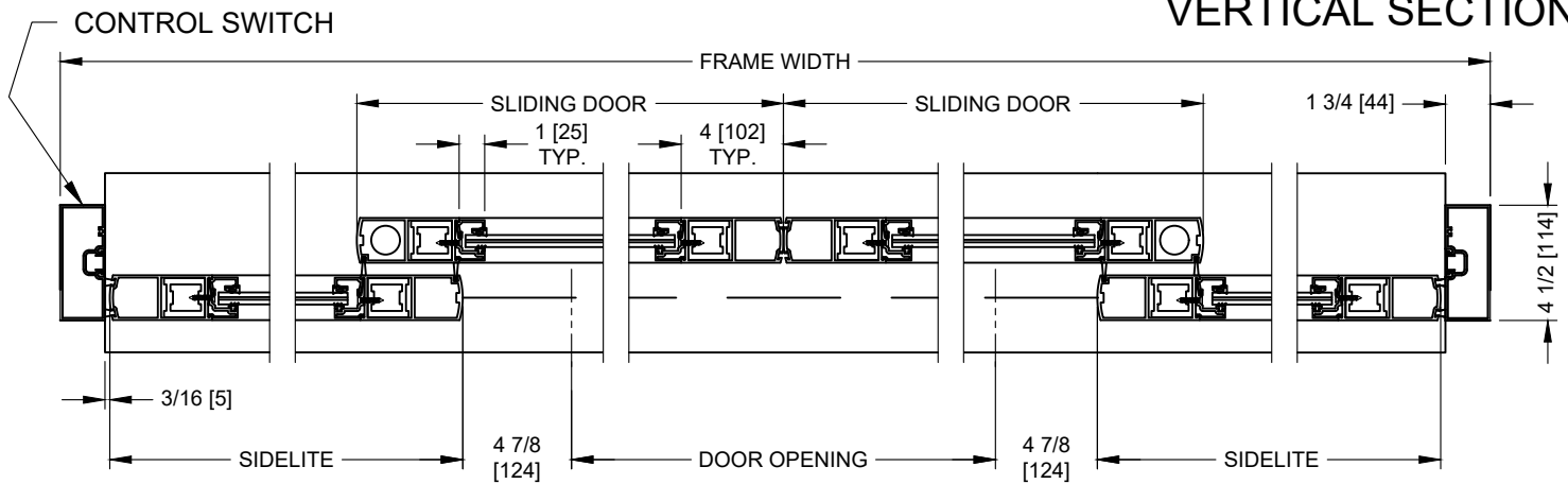
HORIZONTAL SECTION
