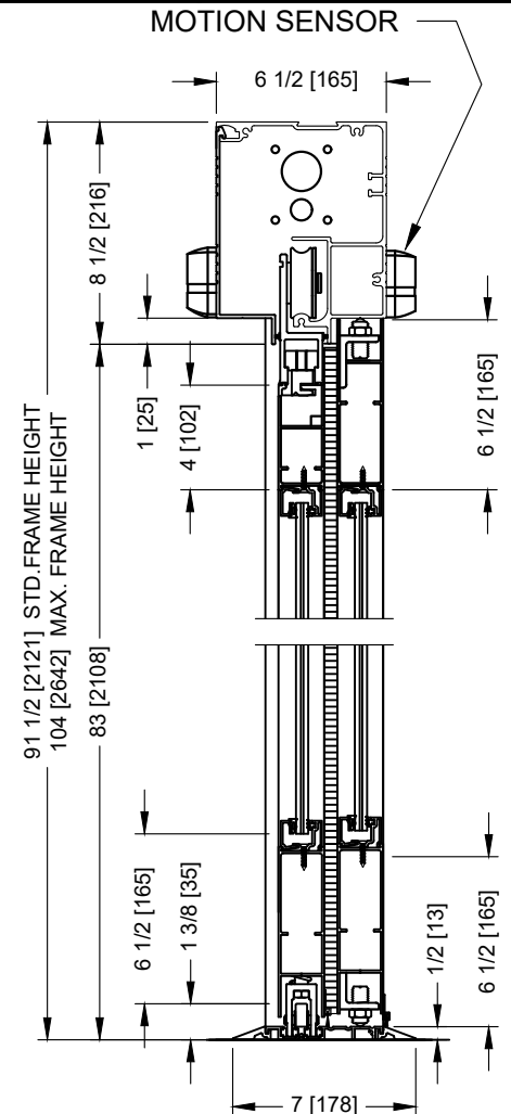
VERTICAL SECTION
