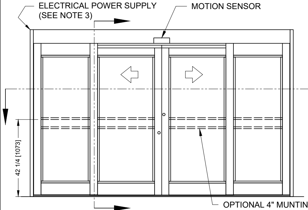
EXTERIOR ELEVATION
