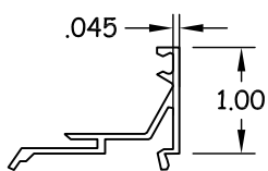
19 GLASS STOP BASE 6063-T5
