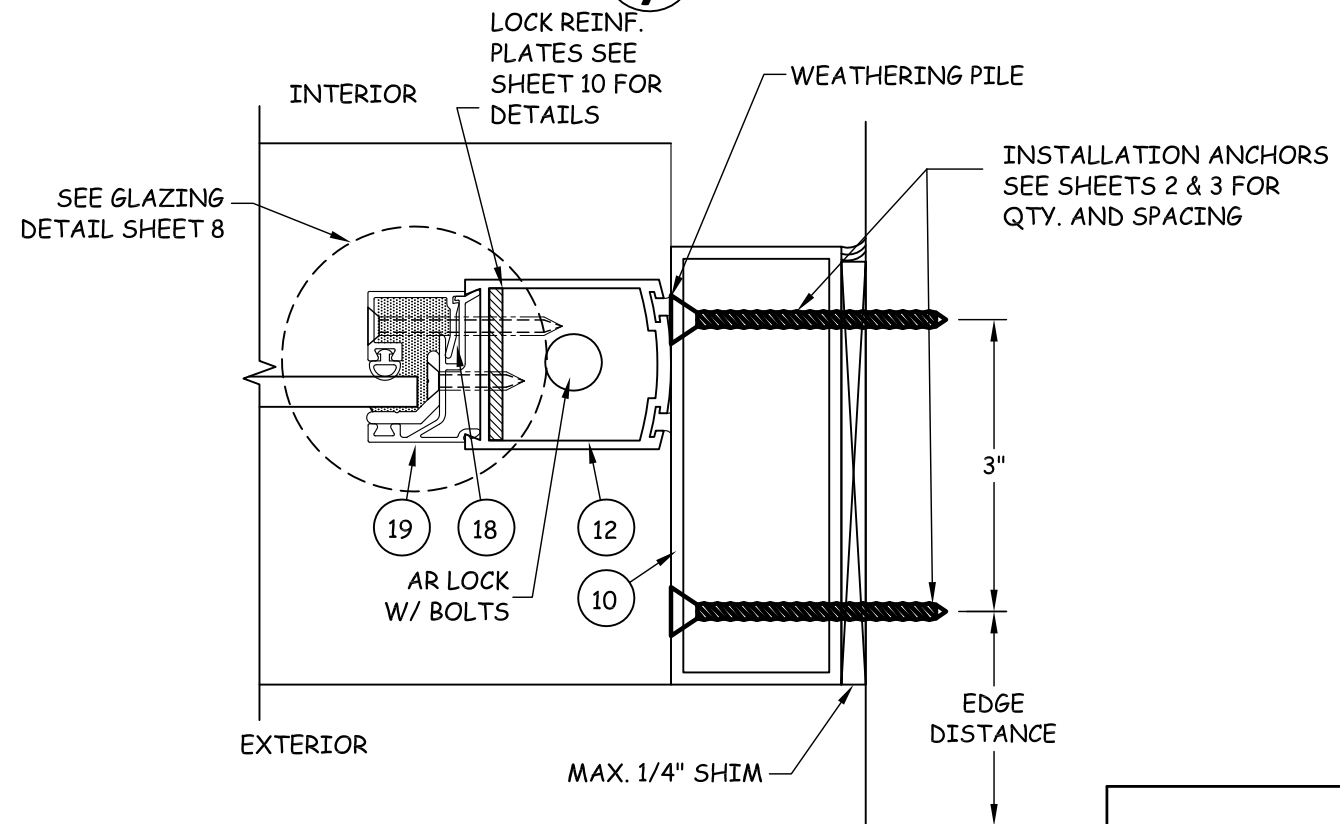
F HORIZONTAL SECTION 7 PANEL INTERLOCK
