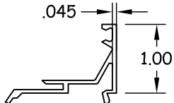
19 GLASS STOP BASE 6063-T5
