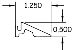
9 THRESHOLD RAMP 6005-T5
