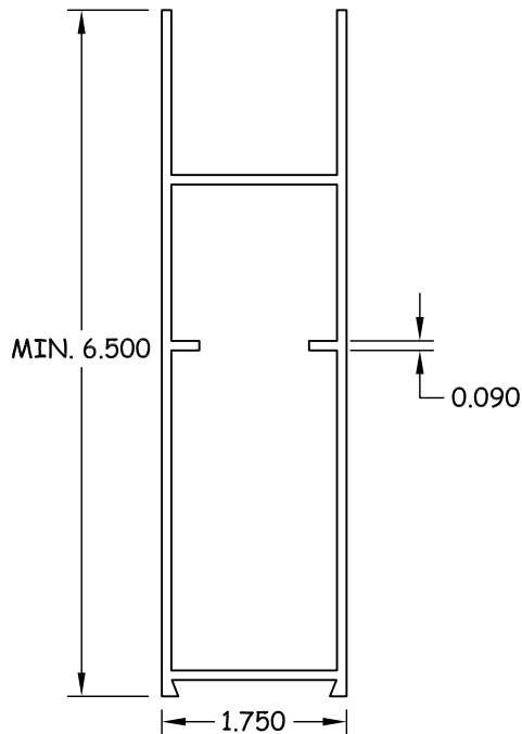
14 TOP RAIL SIDELITE 6063-T6
