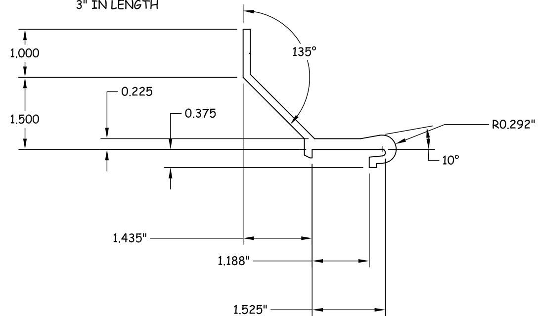
21 ANTI-RISE SUPPORT 6063-T5 3" IN LENGTH
