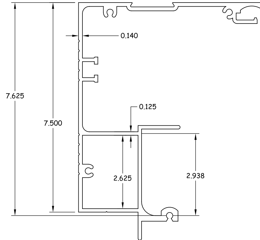
20 1-PIECE HEADER 6063-T5
