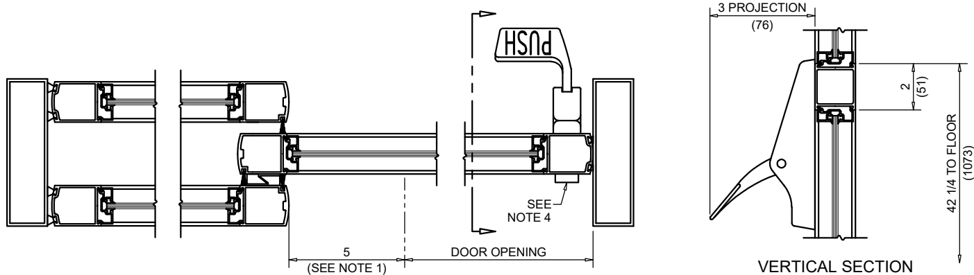
HORIZONTAL SECTION (AT MUNTIN BAR)
