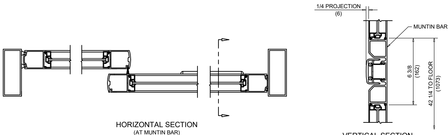
VERTICAL SECTION
