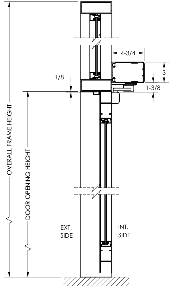
VERTICAL SECTION BUTT/OFFSET PIVOT OPTION
