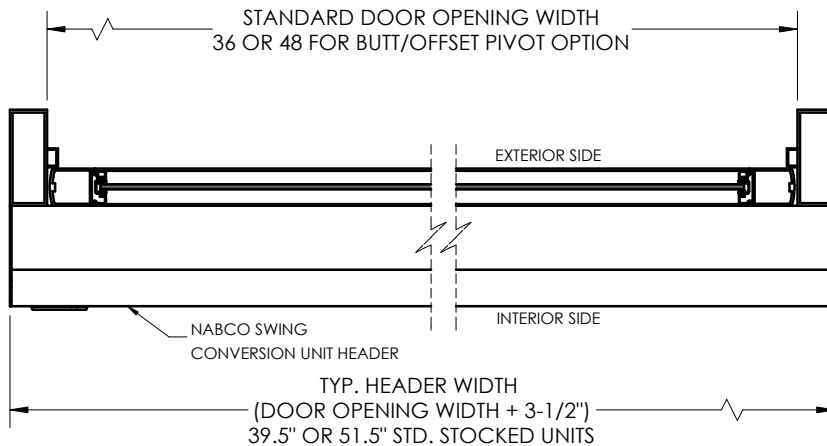
HORIZONTAL SECTION
