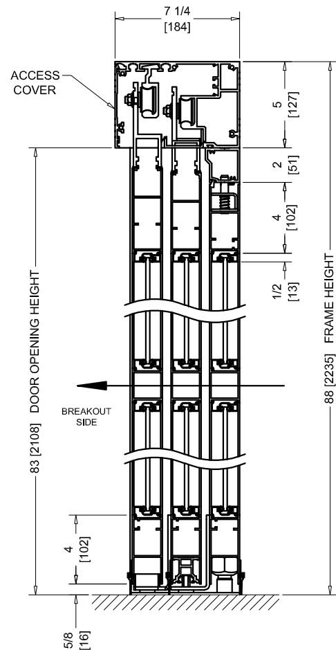
VERTICAL SECTION
