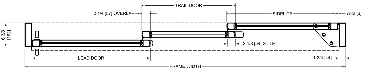
HORIZONTAL SECTION
