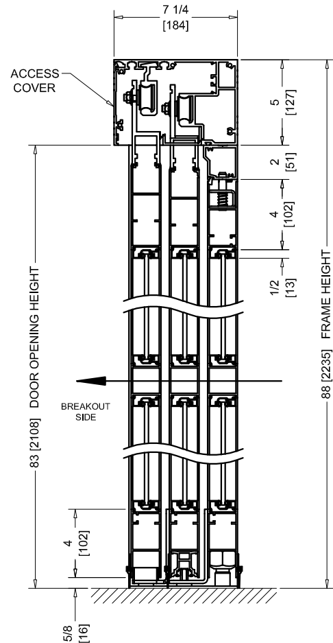
VERTICAL SECTION
