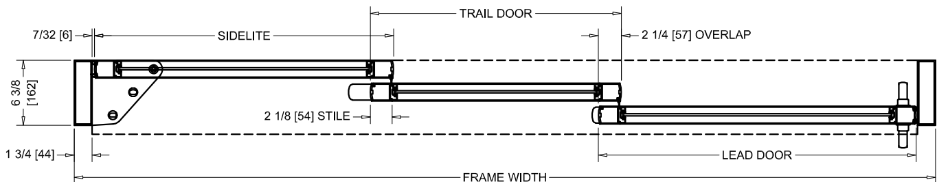
HORIZONTAL SECTION
