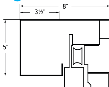
Slim Header Profile
