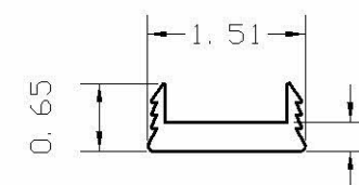
24-2967 RAIL CLIP ALLOY 6063-T5
