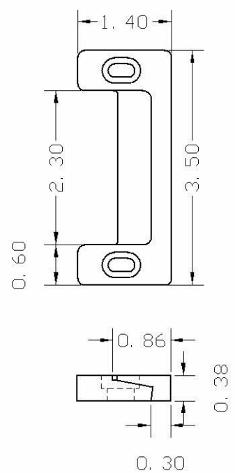
DOOR PANEL INTERLOCK (FEMALE) 24-14043
