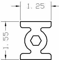
14-13855 LOCKROD GUIDE ALLOY: 6063-T5
