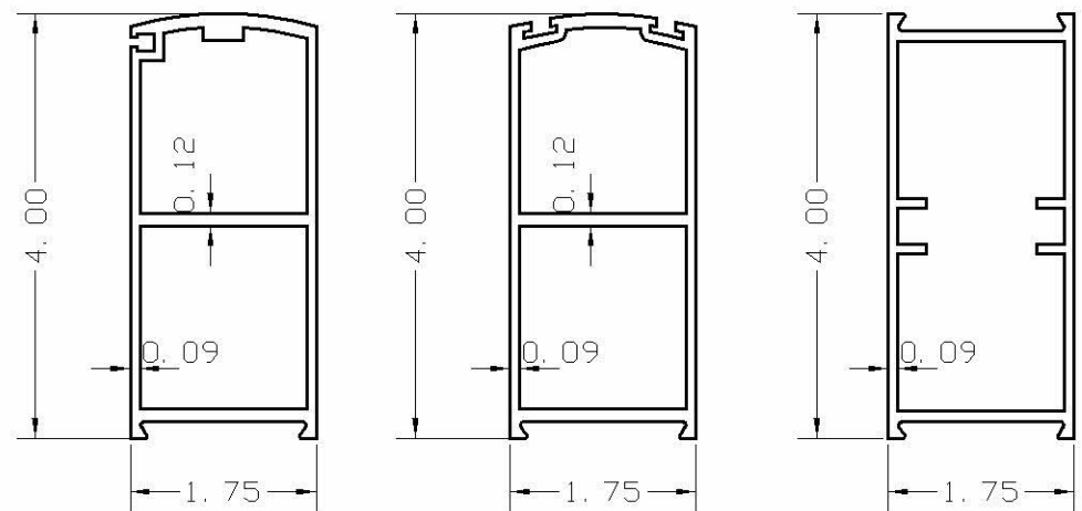
14-13288 4" PIVOT STILE ALLOY: 6063-T5
