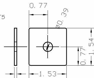
14-9225 TIE ROD BACK-UP PLATE ANSI 1018 STEEL
