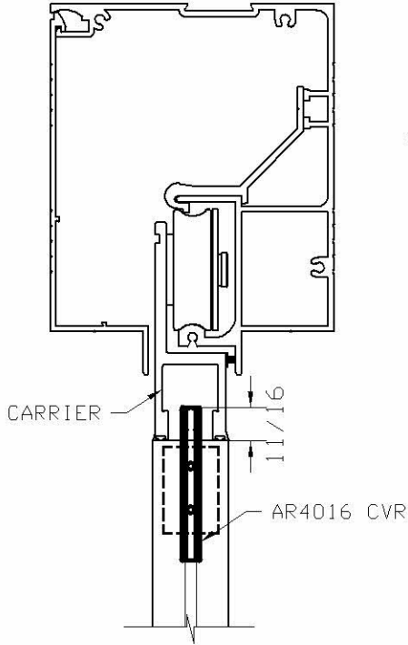
AR 4016 CVR CARRIER ENGAGEMENT
