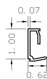
M-X0334 LEVEL D GLASS STOP ALLOY: 6063-T5
