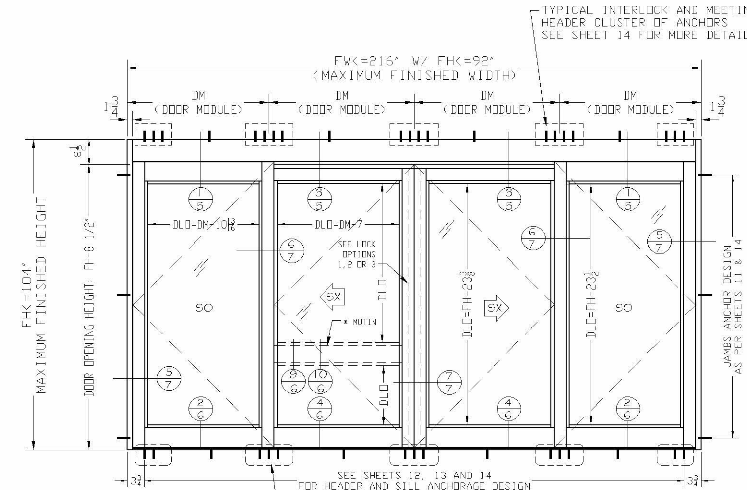
SO SX-SX SO EXTERIOR VIEW
