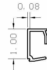
M-X0336 NON IMPACT GLASS STOP ALLOY: 6063-T5
