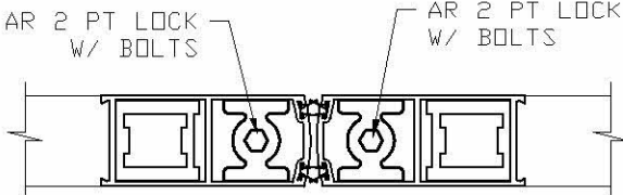
AR 4016 CVR CARRIER ENGAGEMENT
