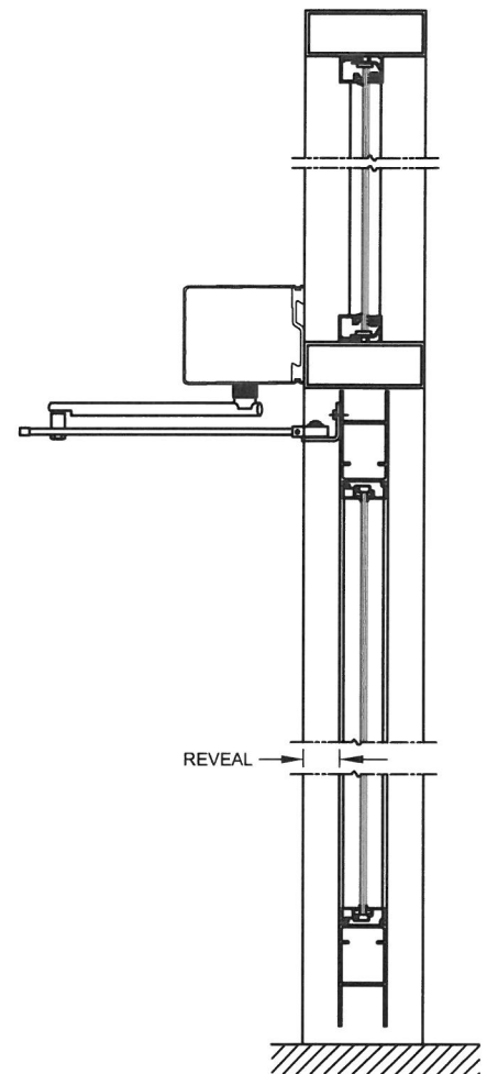
VERTICAL SECTION CENTER PIVOT OPTION
