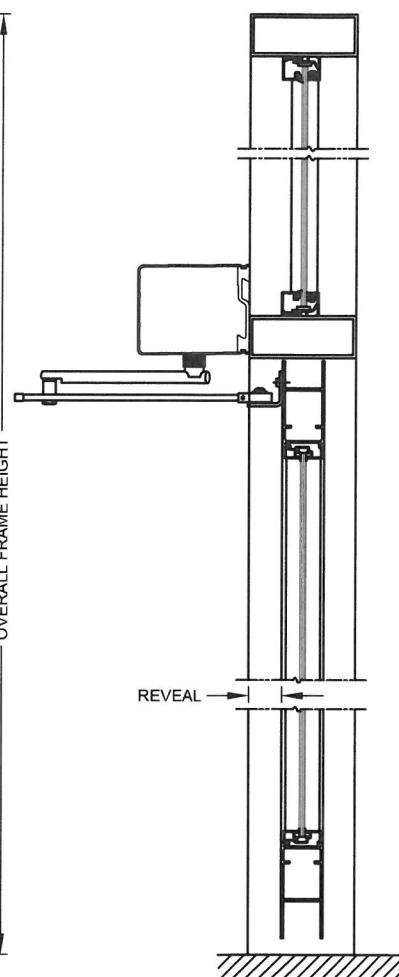
VERTICAL SECTION CENTER PIVOT OPTION
