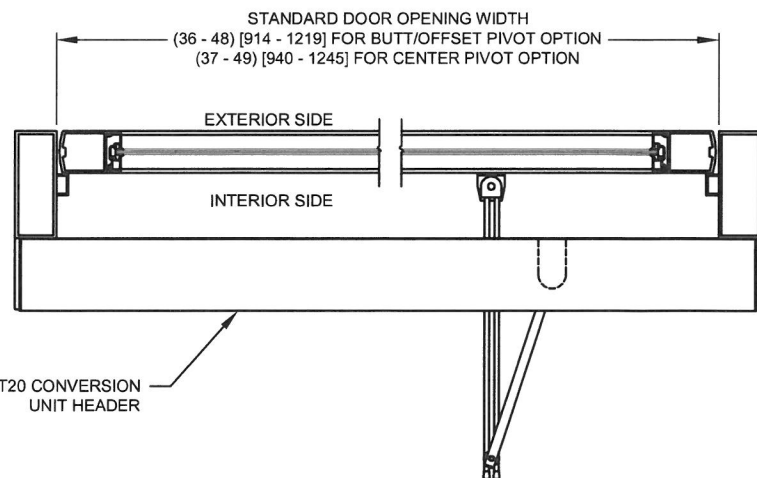
HORIZONTAL SECTION
