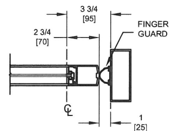
HINGE JAMB AT CENTER PIVOT OPTION
