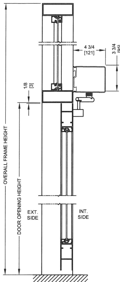
VERTICAL SECTION BUTT/OFFSET PIVOT OPTION
