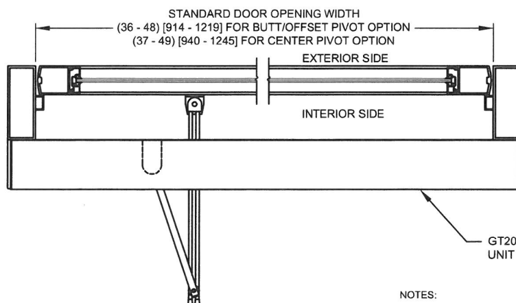
HORIZONTAL SECTION
