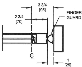
HINGE JAMB AT CENTER PIVOT OPTION
