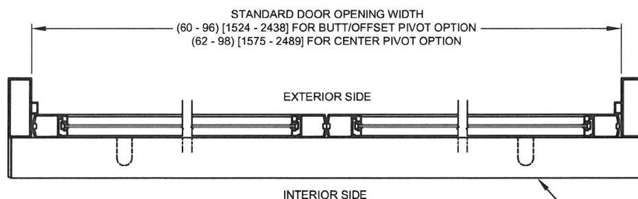
HORIZONTAL SECTION
