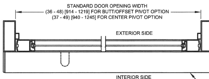
HORIZONTAL SECTION
