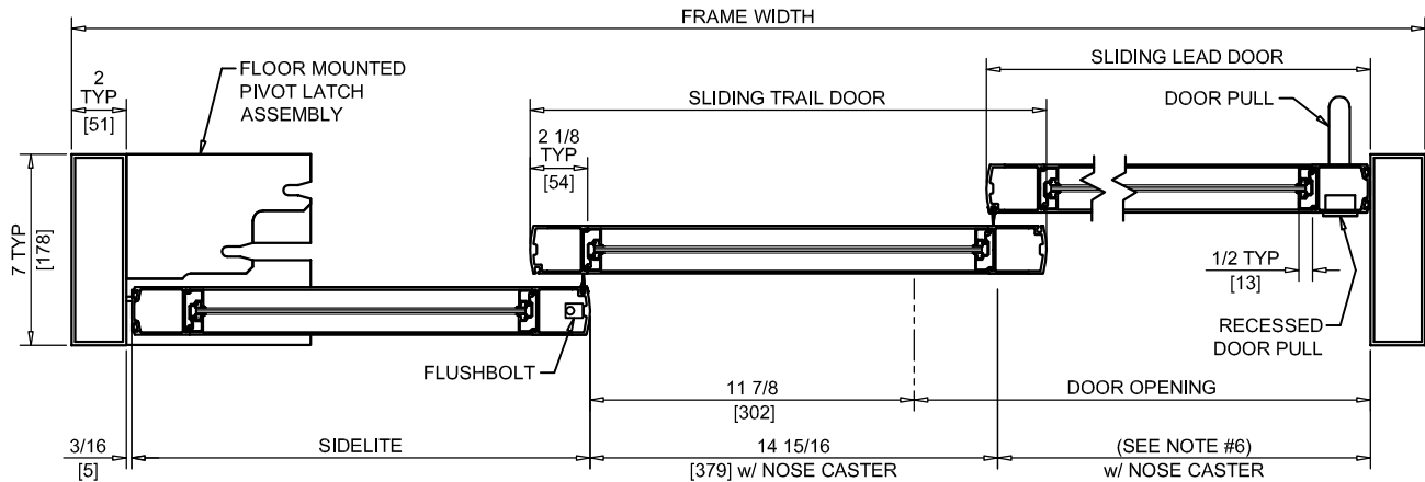
HORIZONTAL SECTION
