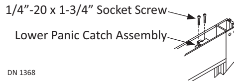
Figure 75 Align the Lower Panic Catch to the Upper Panic Catch
