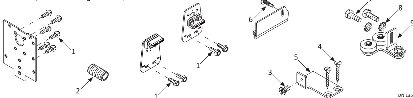
Fixed Sidelite 1175 Parts Kit: LH P/N M-01256 and RH P/N M-01253
