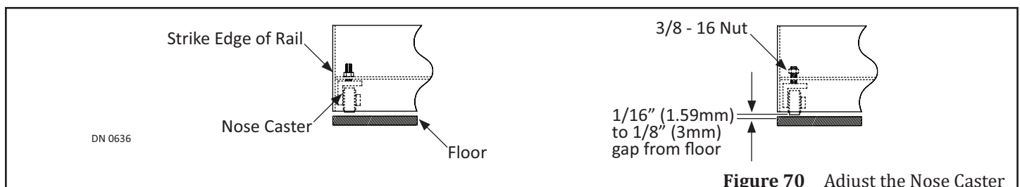
Figure 70 Adjust the Nose Caster
