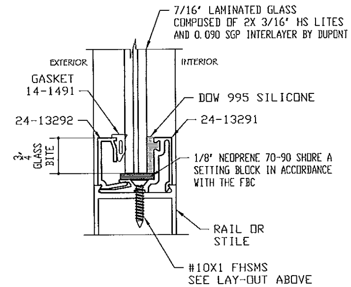
WET GLAZING DETAIL ENTIRE PERIMETER ALL LITES LARGE & SMALL IMPACT
