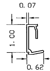
24-13292 GLASS STOP ALLOY: 6063-T5
