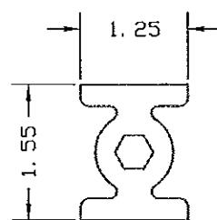
14-13855 LOCKROD GUIDE ALLOY: 6063-T5
