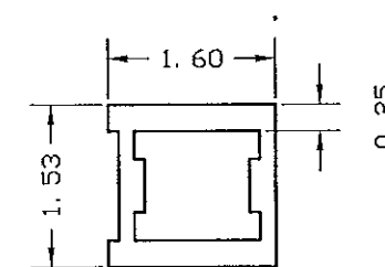
14-13950 ALUMINUM STIFFENER ALLOY 6063-T5
