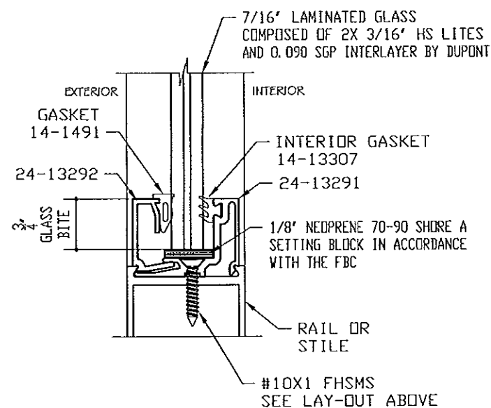
DRY GLAZING DETAIL ENTIRE PERIMETER ALL LITES LARGE & SMALL IMPACT
