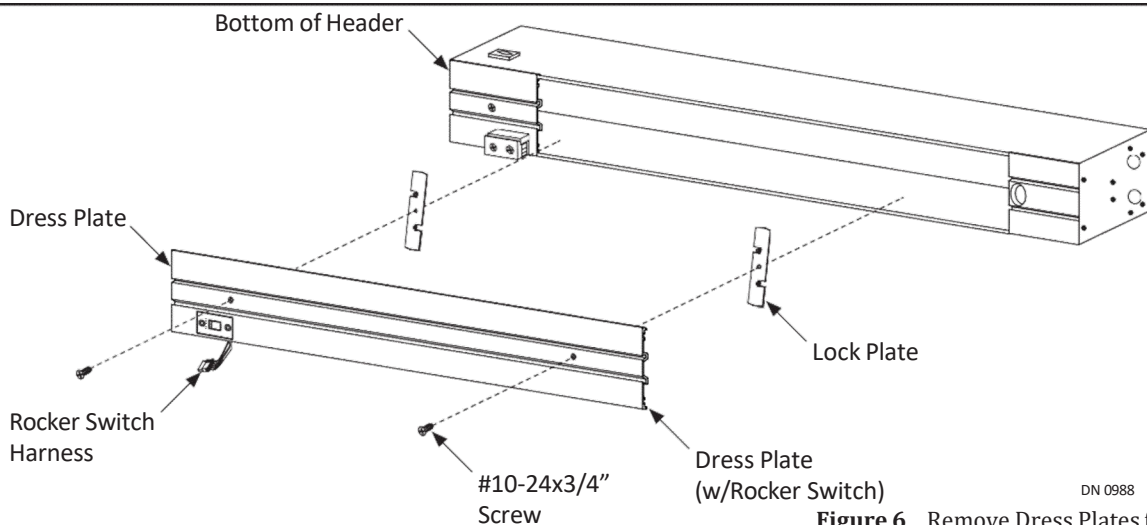
Figure 6 Remove Dress Plates from Header
