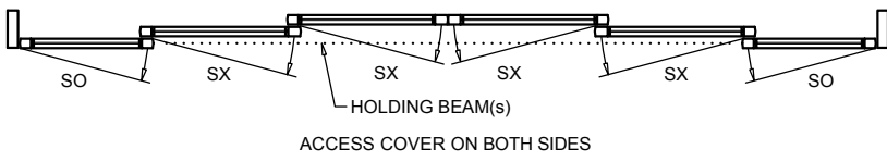
EXTERIOR ELEVATION/PLAN
