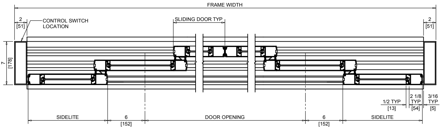
HORIZONTAL SECTION
