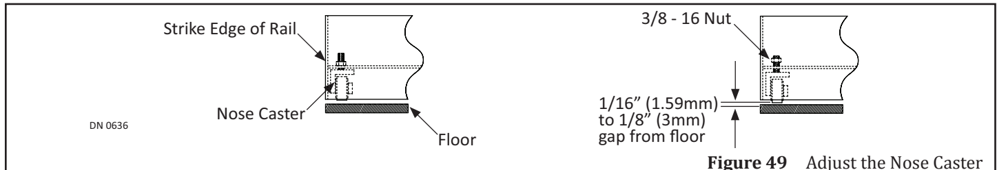
Figure 49 Adjust the Nose Caster
