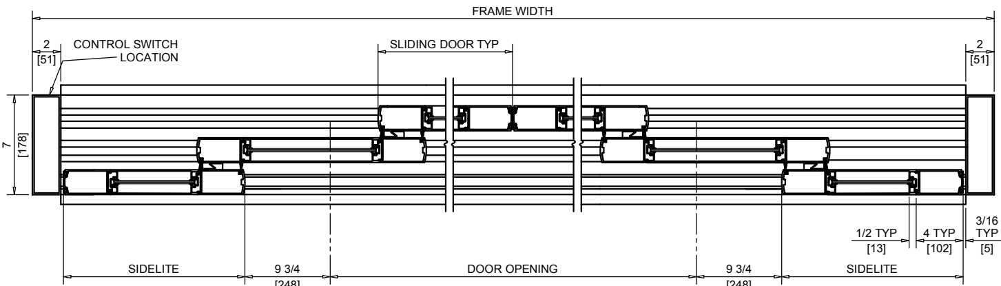
HORIZONTAL SECTION
