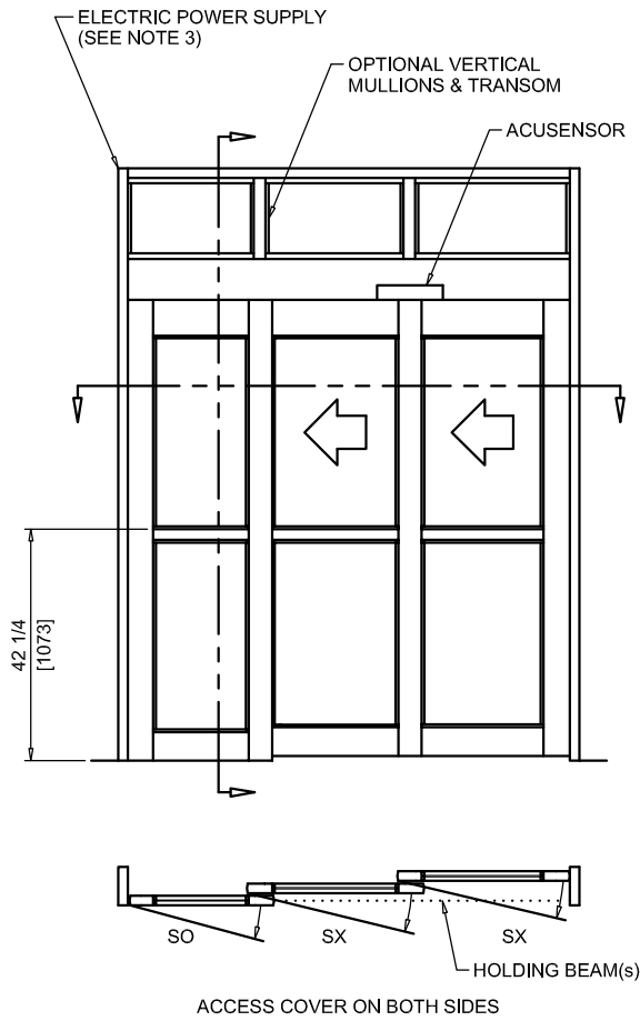
EXTERIOR ELEVATION/PLAN
