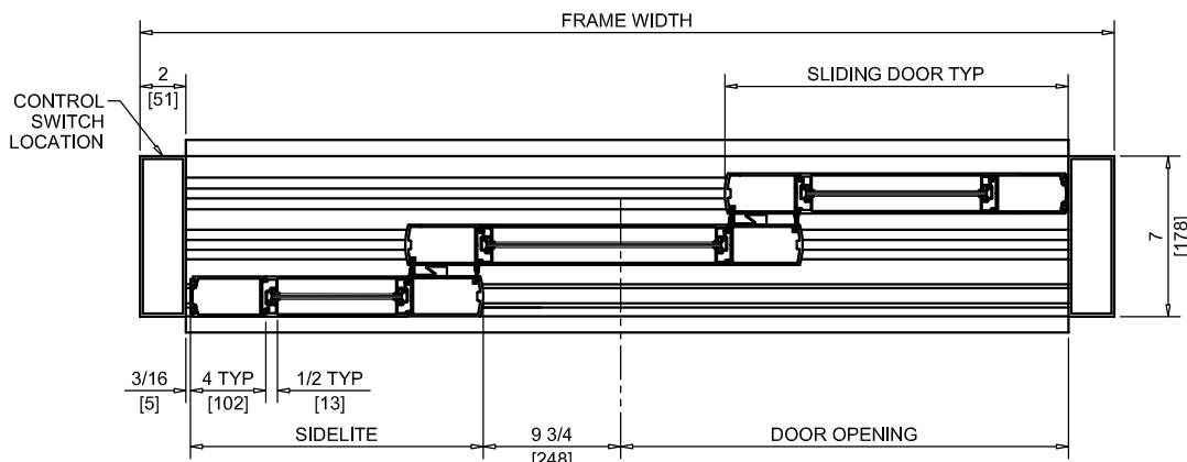
HORIZONTAL SECTION
