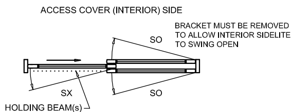
EXTERIOR ELEVATION/PLAN
