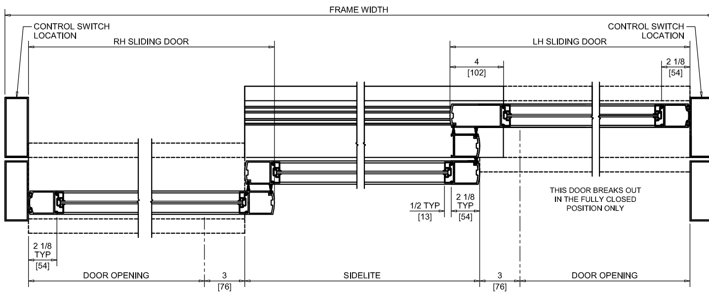
HORIZONTAL SECTION
