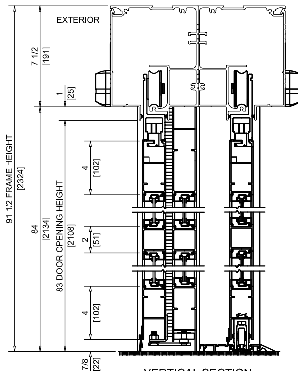
VERTICAL SECTION (SHOWN WITH BOTH DOORS OPEN)
