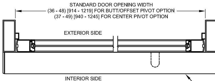
HORIZONTAL SECTION
