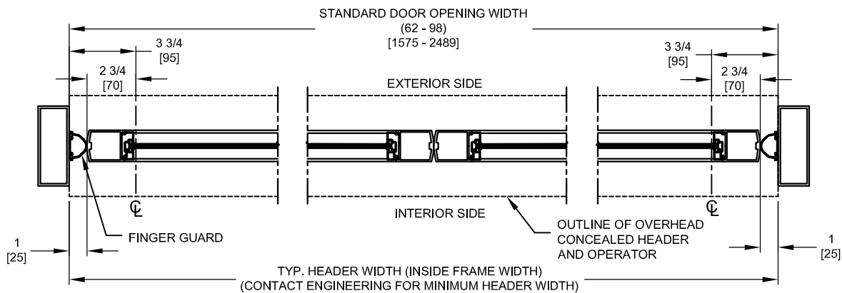
HORIZONTAL SECTION
