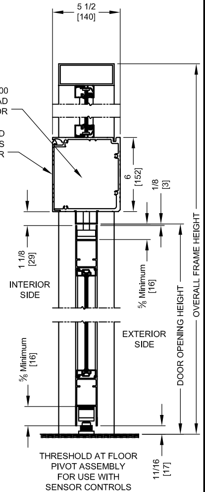
VERTICAL SECTION
