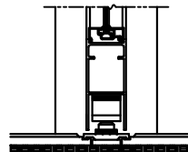
THRESHOLD AT FLOOR PIVOT ASSEMBLY FOR USE WITH MAT CONTROLS
