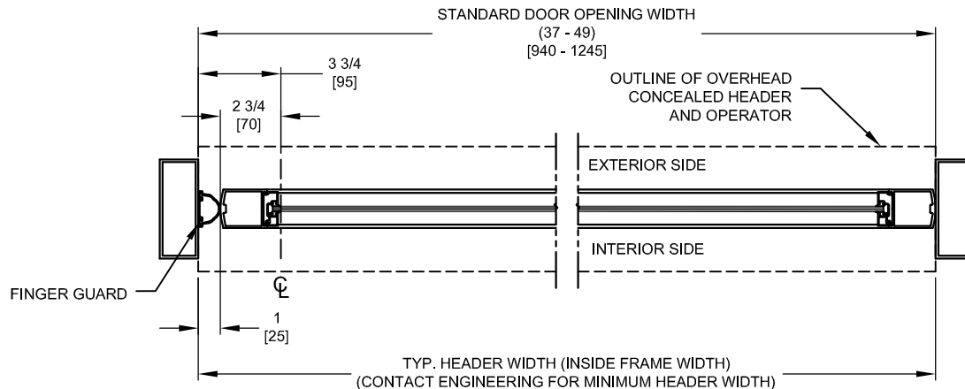
HORIZONTAL SECTION
