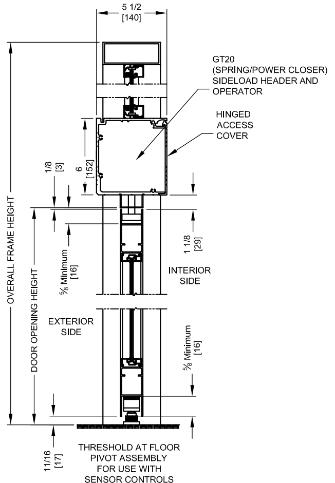
VERTICAL SECTION
