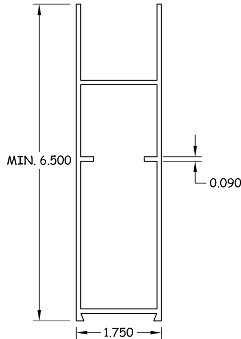
14 TOP RAIL SIDELITE 6063-T6
