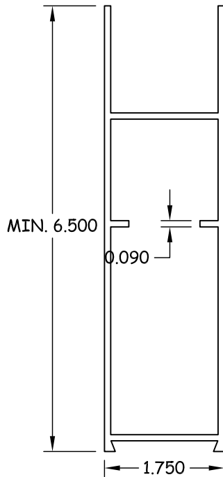
14 TOP RAIL SIDELITE 6063-T6
