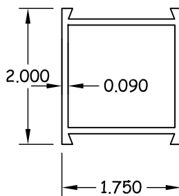
13 FIXED VERT. STILE 6063-T6
