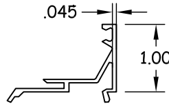
19 GLASS STOP BASE 6063-T5
