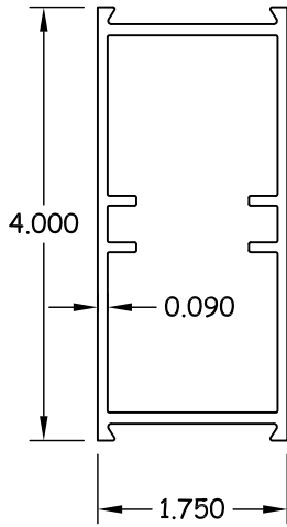
6 4" FIXED VERT. STILE 6063-T6
