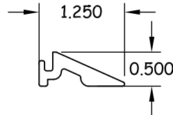
9 THRESHOLD RAMP 6005-T5
