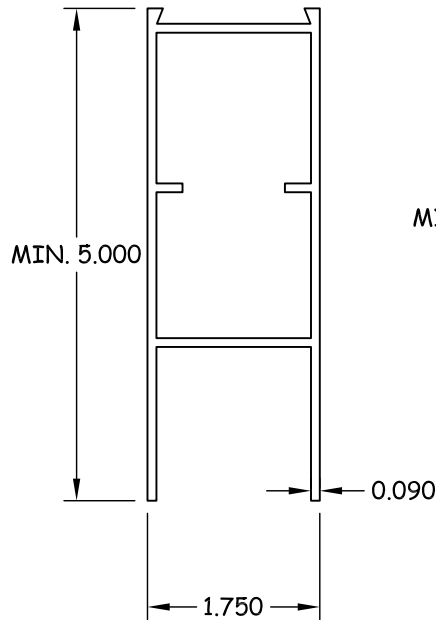
15 BOTTOM RAIL SIDELITE 6063-T6
