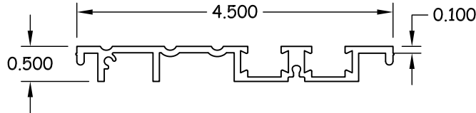
9 THRESHOLD RAMP 6005-T5
