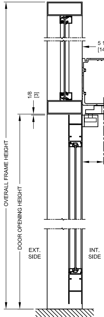
VERTICAL SECTION BUTT/OFFSET PIVOT OPTION
