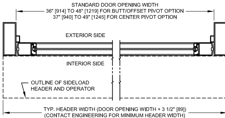
HORIZONTAL SECTION
