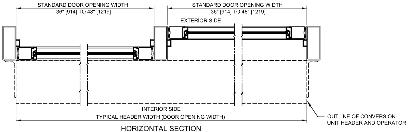
HORIZONTAL SECTION
