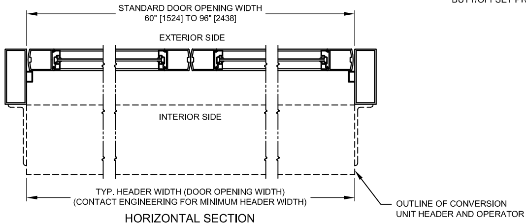
HORIZONTAL SECTION
