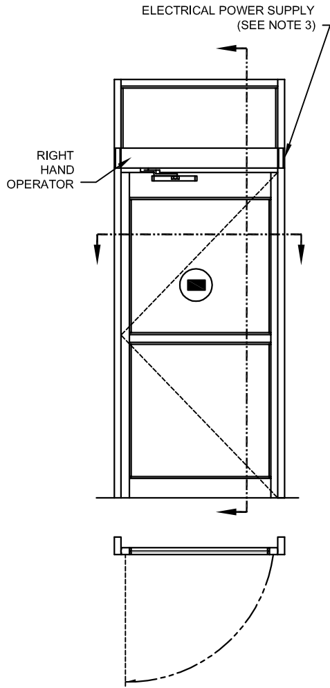
INTERIOR ELEVATION
