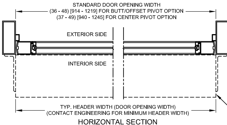
HORIZONTAL SECTION
