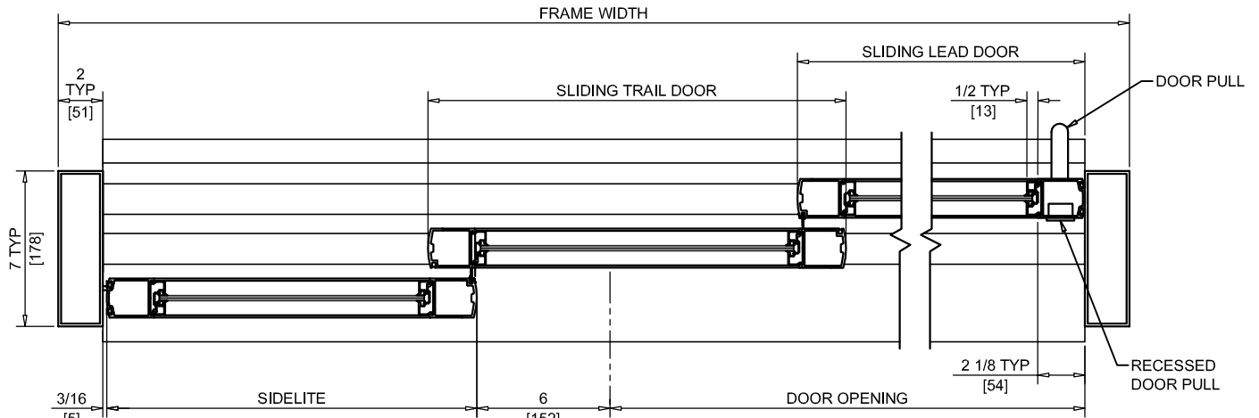
HORIZONTAL SECTION
