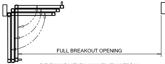
BREAKOUT PLAN/ ELEVATION ACCESS COVER ON NON-BREAKOUT SIDE
