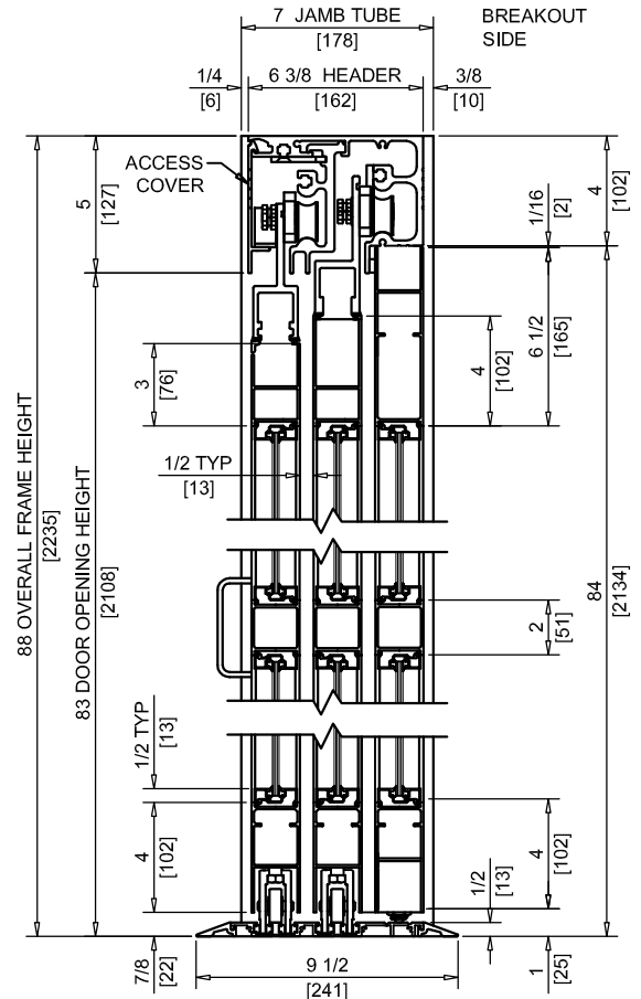
VERTICAL SECTION (WITH DOOR OPEN)
