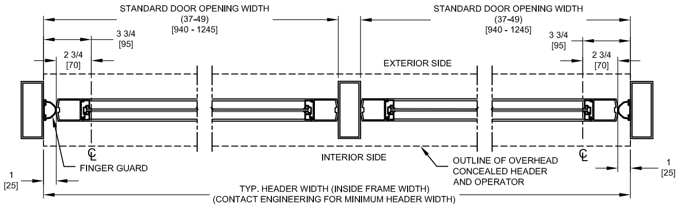
HORIZONTAL SECTION
