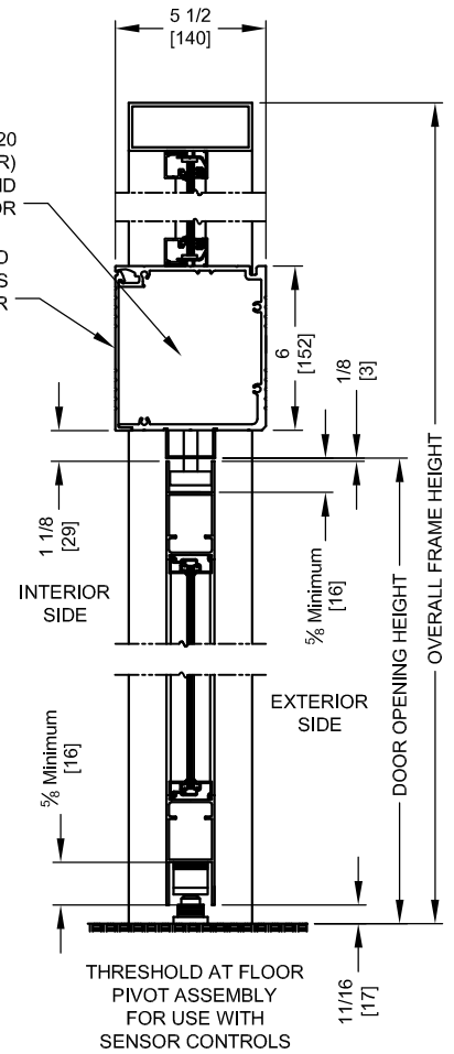
VERTICAL SECTION
