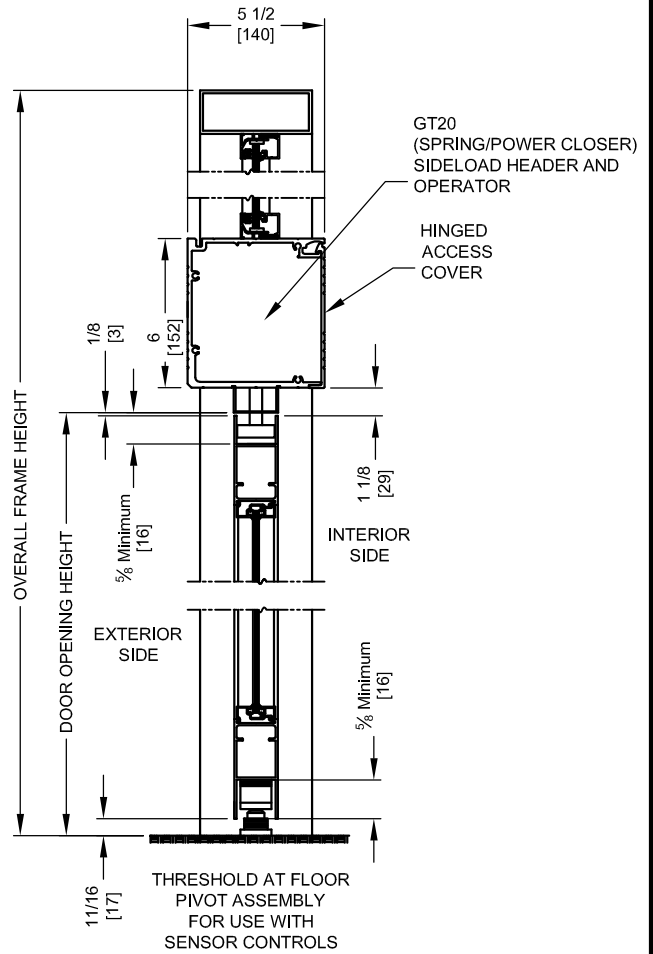
VERTICAL SECTION
