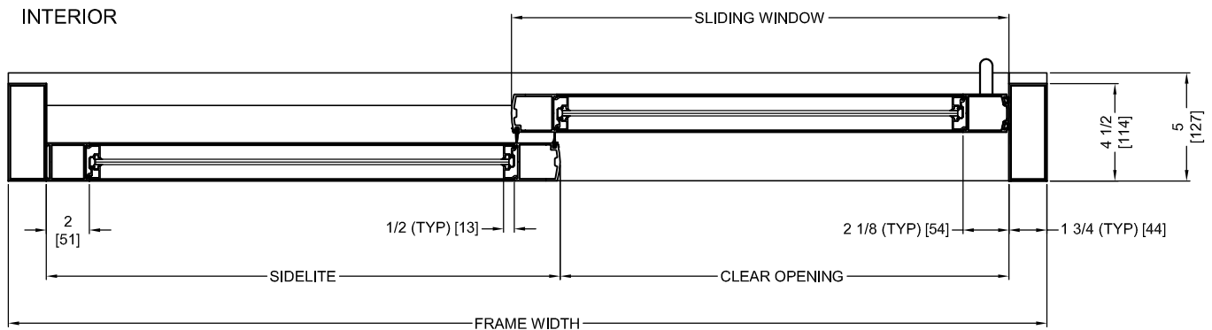
HORIZONTAL SECTION
