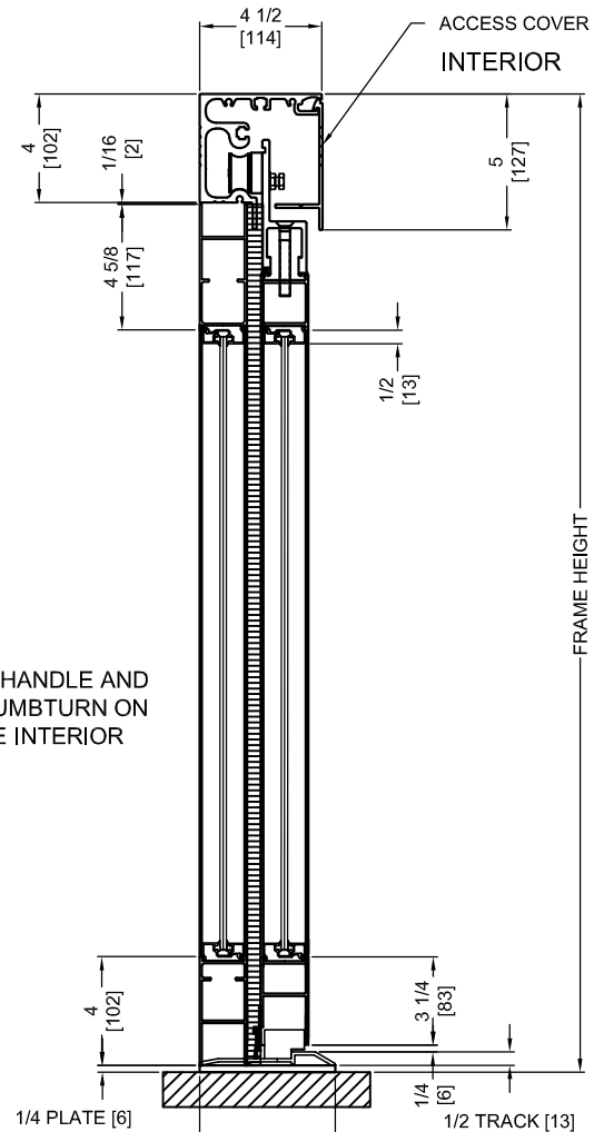
VERTICAL SECTION (WITH WINDOW OPEN)
