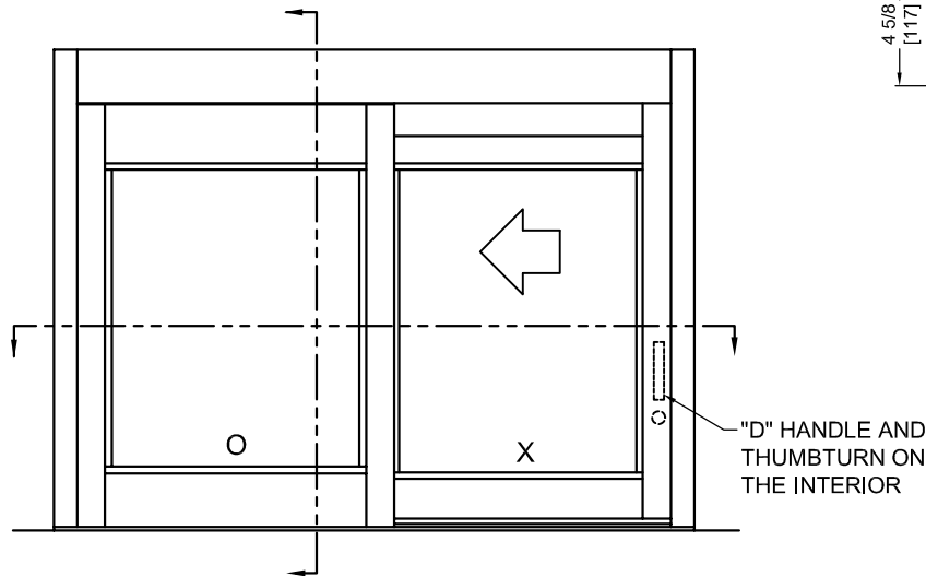
EXTERIOR ELEVATION
