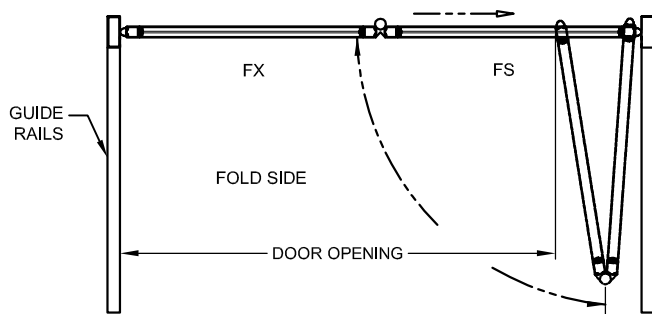
EXTERIOR ELEVATION/PLAN
