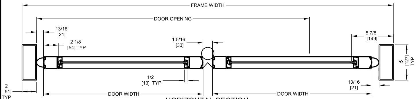
HORIZONTAL SECTION
