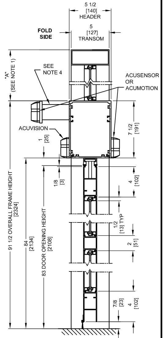
VERTICAL SECTION
