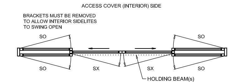
EXTERIOR ELEVATION/PLAN
