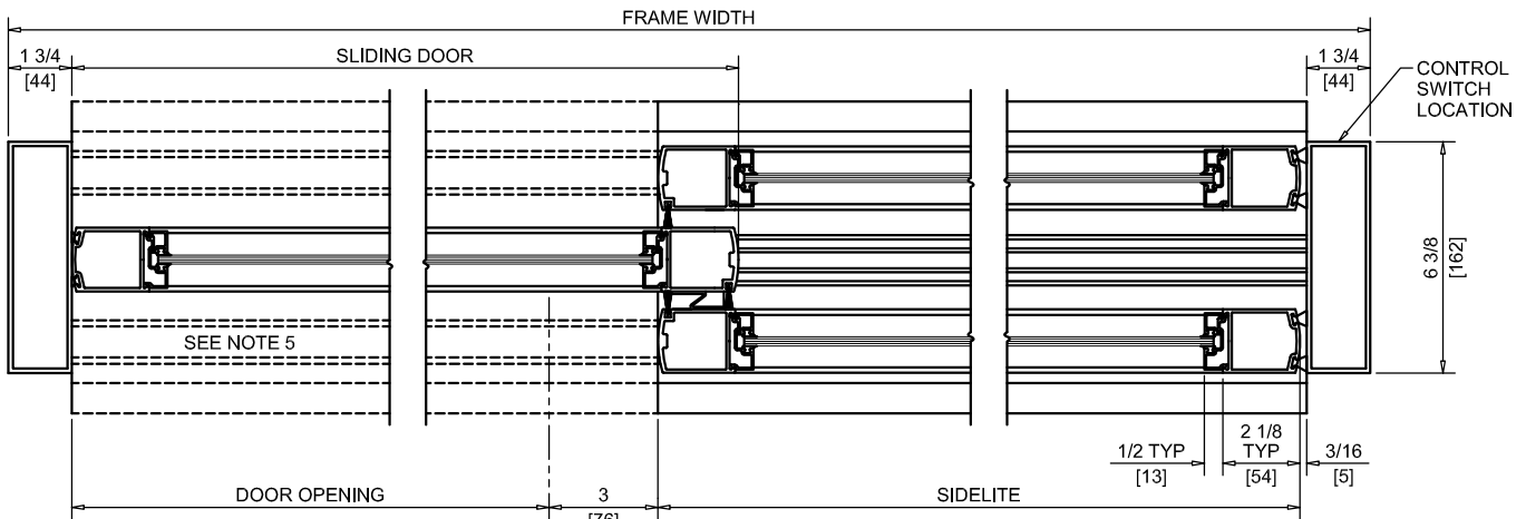
HORIZONTAL SECTION
